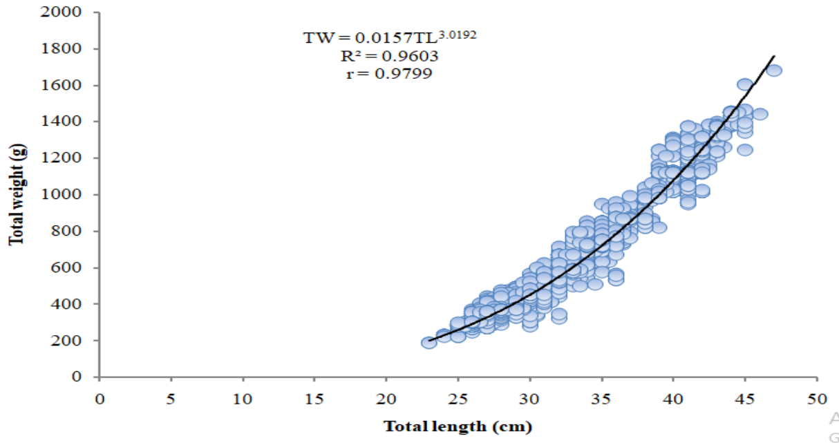
Figure 3: Length-weight relationship of pooled O. niloticus in Lake Abaya.
