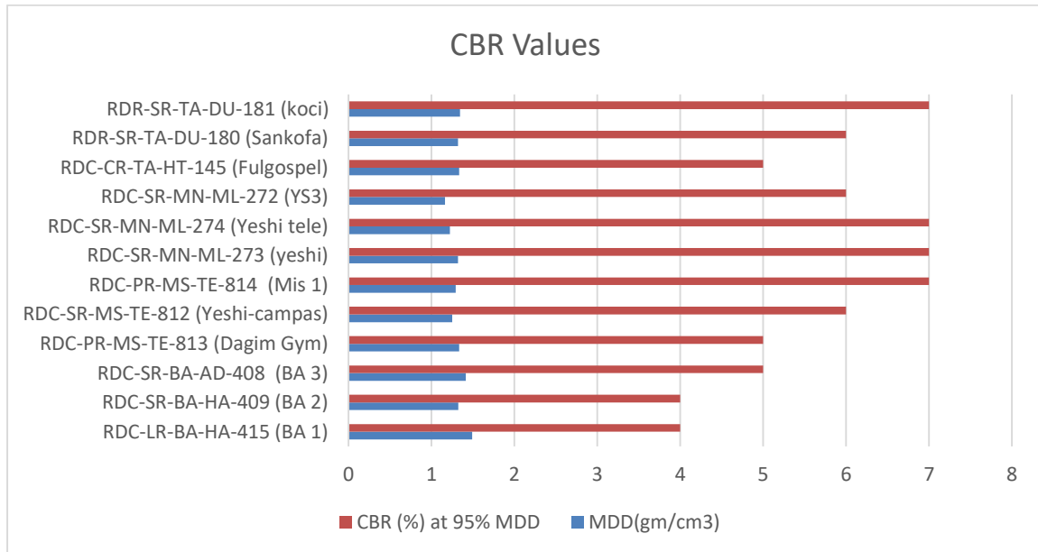
Figure 4. Laboratory Test CBR values of study area sub cities
