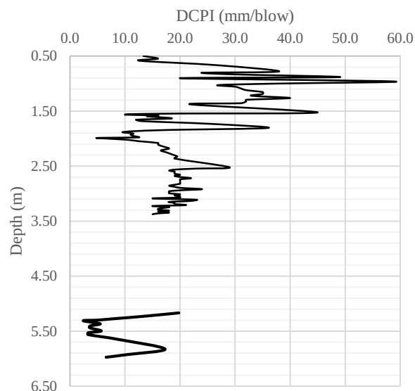
Figure 8. Result of DCP test at the pit excavation site
