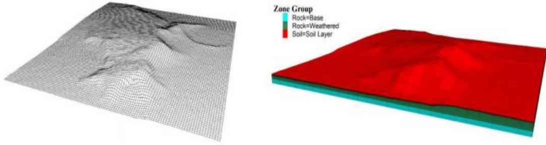
Figure 7. Numerical Model geometric layer and computation zones
