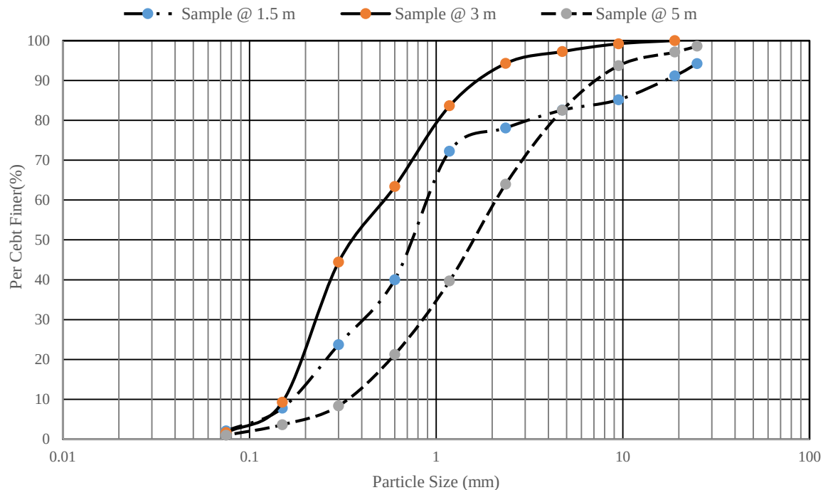
Figure 9. Particle Size Distribution of Soil Samples from Pit Excavation
