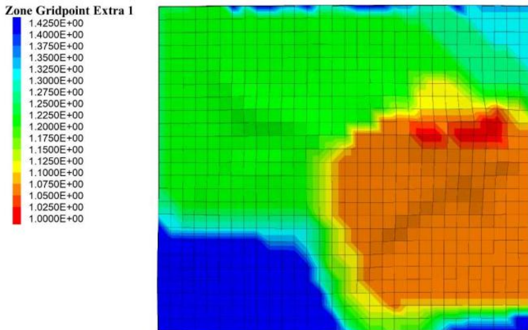
Figure 13. Factor of Safety contours for 'wet' condition
