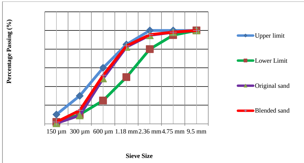
Figure 1. Gradation result of the original sand samples and blended sand sample of Belate area sand.
