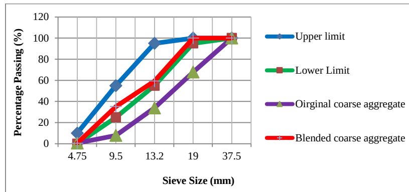
Figure 4. Gradation chart of the original sample and blended coarse aggregate of Monopol area coarse aggregate
