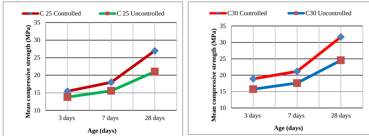
(a) Compressive strength development of C-25 MPa grade of concrete
