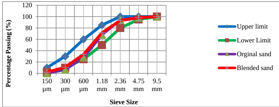
Figure 3. Gradation chart of blended and unblended sand of Hawassa Ayer Marfia sand
