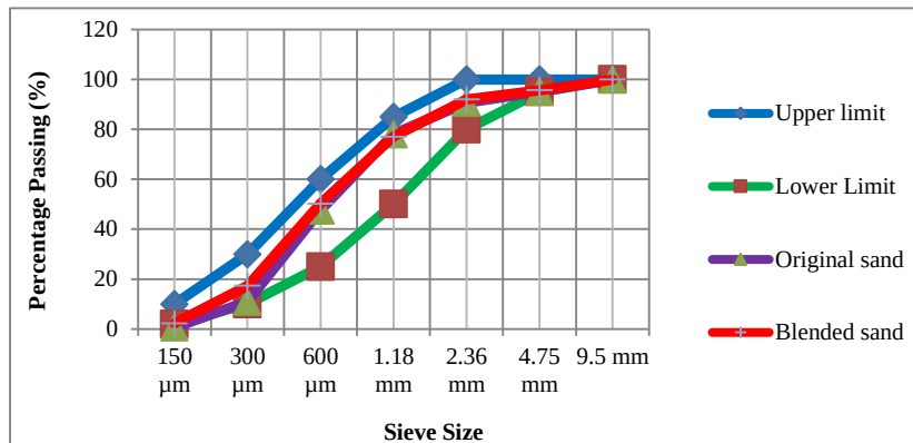
Figure 2: Gradation result of the original sand samples and blended sand sample of Halaba area sand.
