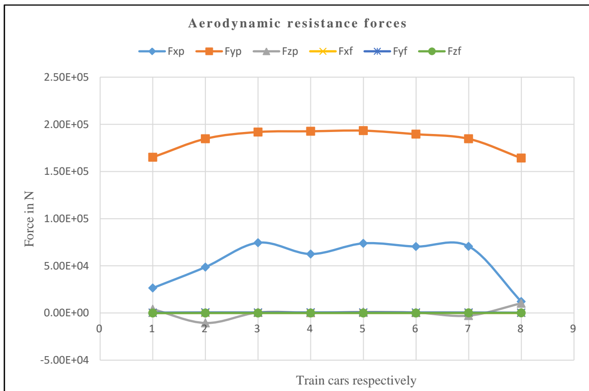
Figure 11. Comparison of the aerodynamic resistance forces value for each car at \beta = 30^\circ
