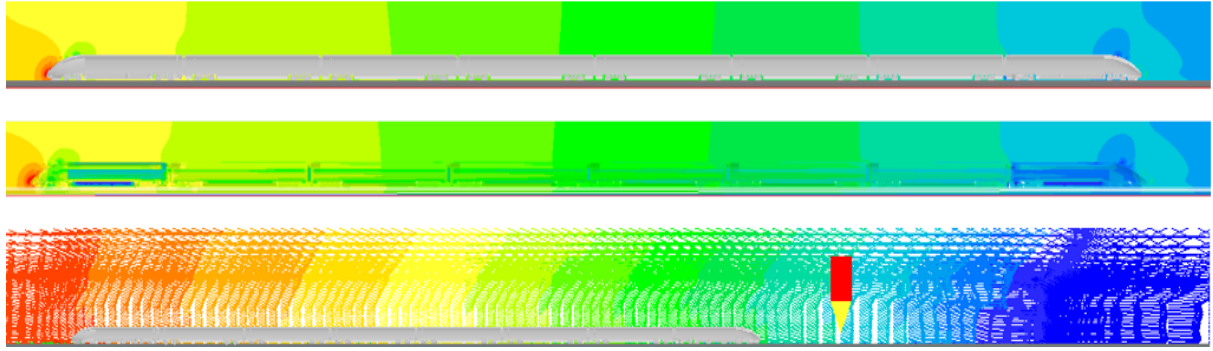
Figure 8. Aerodynamic resistance load distribution on ICE3 full-scaled train at yaw-angle \beta = 15^\circ
