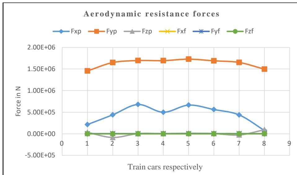
Figure 15. Comparison of the aerodynamic resistance forces value for each car at \beta = 60^\circ
