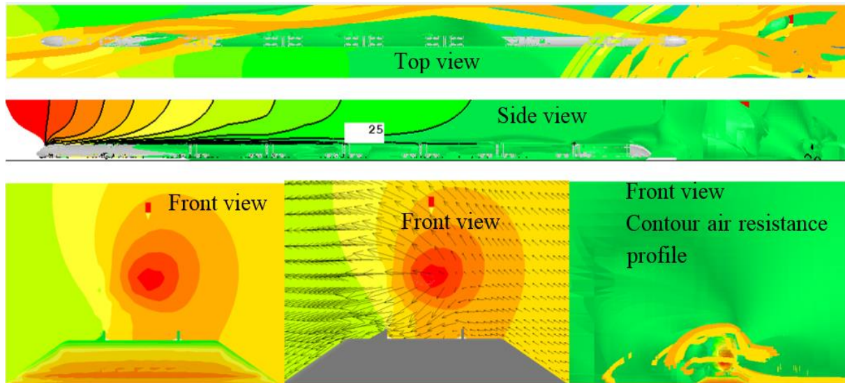
Figure 10. Aerodynamic resistance load distribution on ICE3 full-scaled train at yaw-angle \beta = 30^\circ
