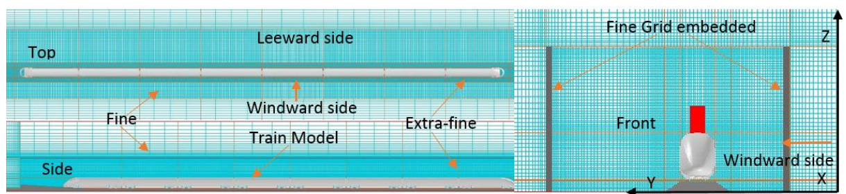
Figure 5. Overall grid structure for test from front and side views
