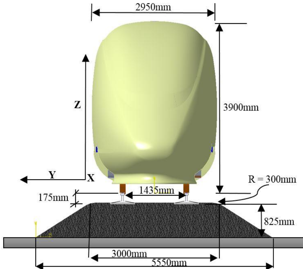
Figure 3. The standard aerodynamics test on a single-track sectional views and ICE 3 high-speed train front side.
