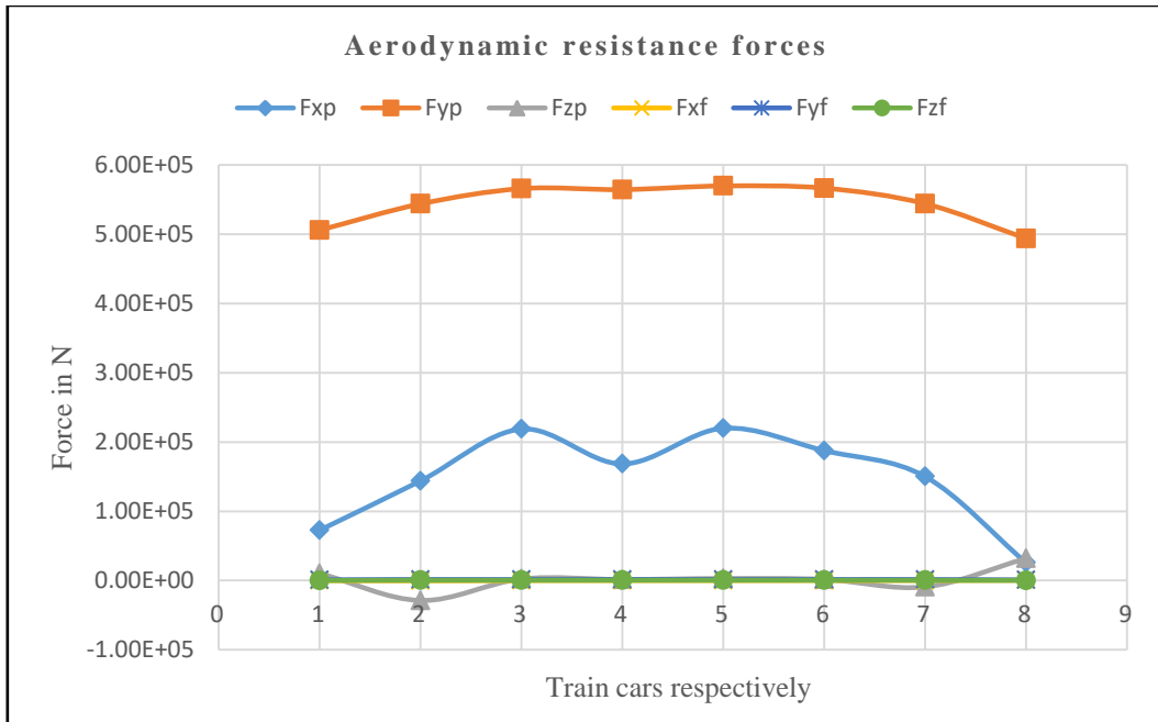
Figure 13. Comparison of the aerodynamic resistance forces value for each car at \beta = 45^\circ
