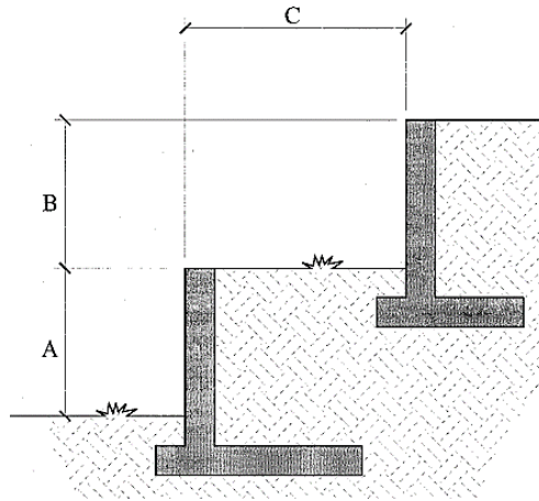
Figure 16. Geometric elements of Stacked Retaining Walls (Weight, 2008)
