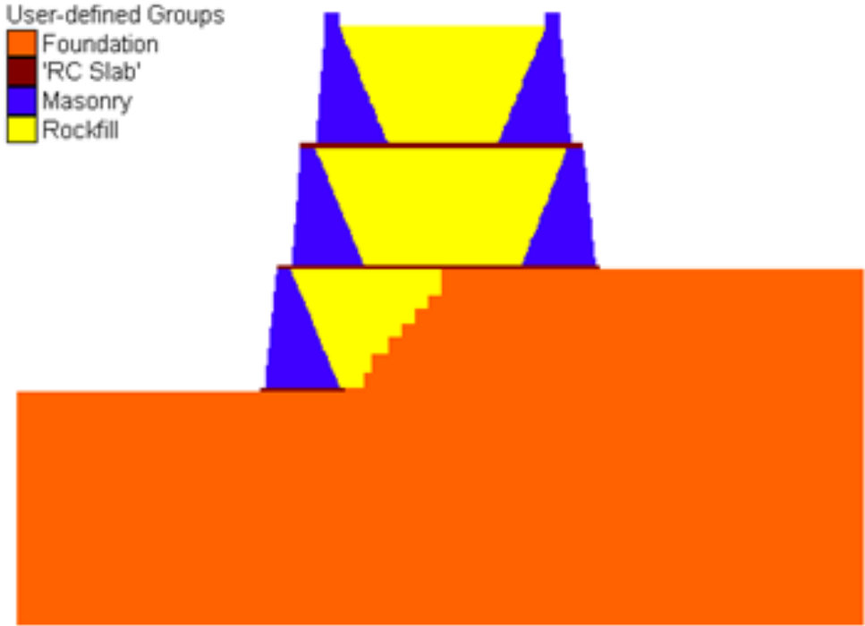
Figure 13. FLAC Model for Previously Recommended Solution
