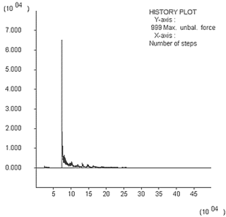
Figure 7. History Plot of Unbalanced for Logita As-Is
