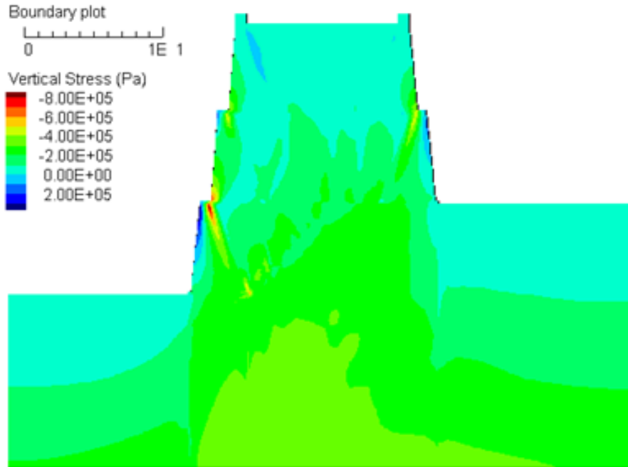
Figure 14. Total Vertical Stress Plot for Previously Recommended Solution
