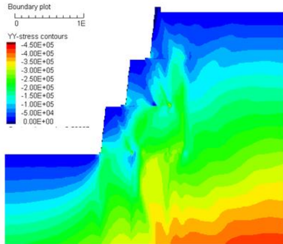
Figure 17. Total Vertical Stress Plot for 1 m offset Logita-Design
