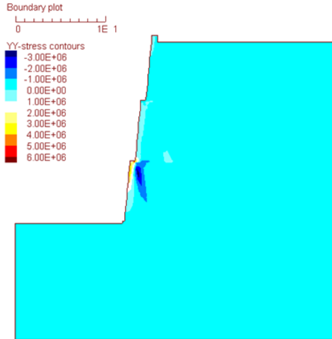
Figure 11. Total Vertical Stress plot for Logita-Design
