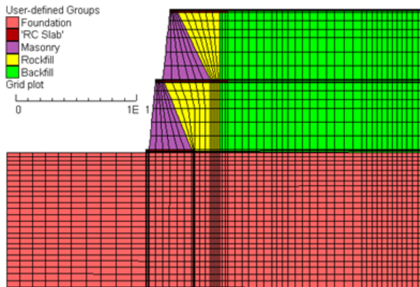
Figure 5. Finite Difference Model for Logita AS-IS
