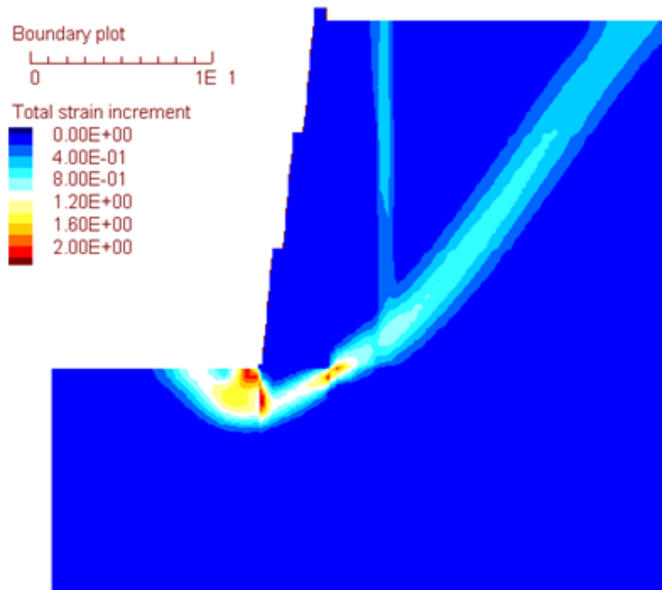
Figure 12. Total Strain Plot for Logita-Design
