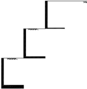
(b) Stacked Cantilever Walls
