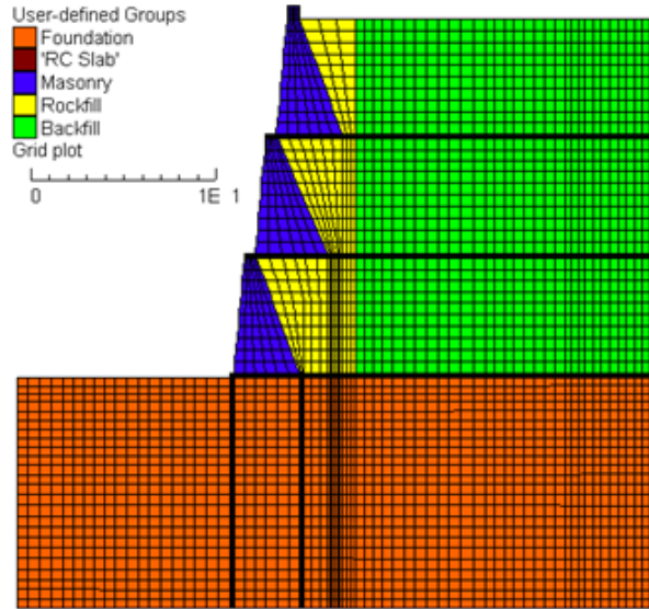
Figure 6. Finite Difference Model Logita –Design
