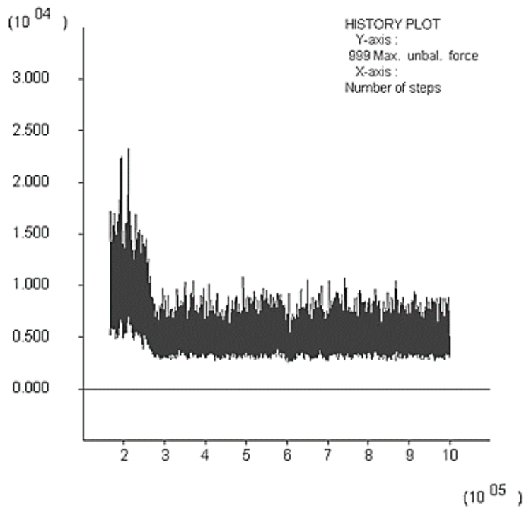
Figure 10. Unbalance force History plot for Logita-Design
